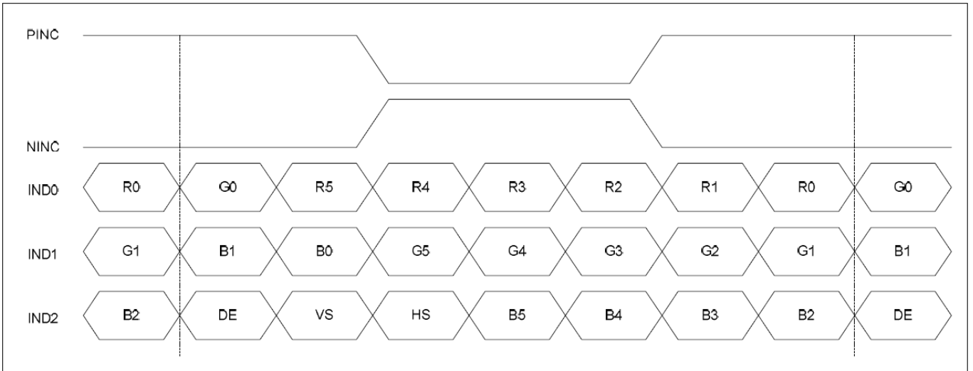
Figure: 6-bit LVDS input
