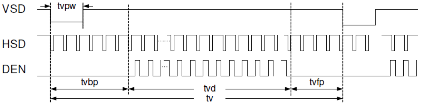
Figure: Vertical input timing diagram
