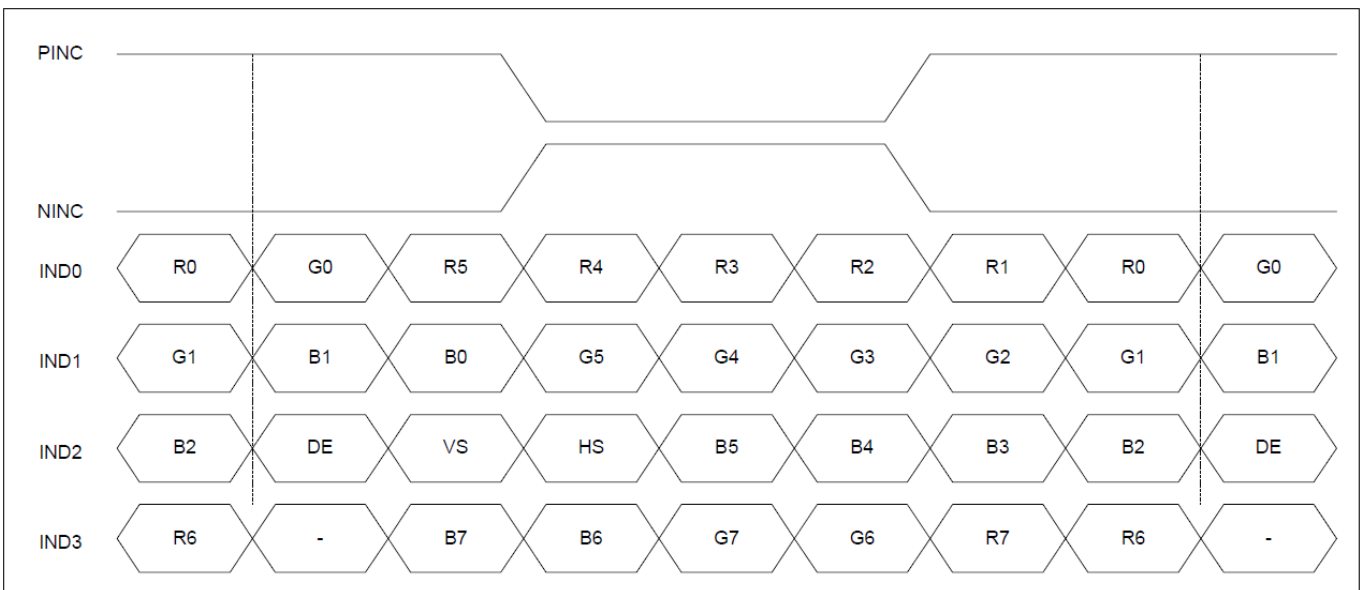
Figure: 8-bit LVDS Input
